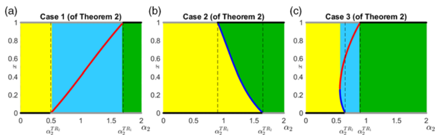
FIGURE 3. Bifurcation diagrams with bifurcation parameter \alpha_2 varying in [0, 2] . The equilibria of offshoring and reshoring, say E_0 and E_1 , are in black if stable and in gray if unstable. Inner equilibria are represented in the blue (unstable) and red (stable) curves as \alpha_2 increases. For each value of \alpha_2 in [0, 2] , the basin of attraction of the reshoring equilibrium E_1 is represented in green, in yellow that of the offshoring equilibrium E_0 , and in azure the basin of the interior equilibrium (red curve). The bifurcation value for the offshoring equilibrium \alpha_2^{TR_2} (transcritical bifurcation) is indicated by a black dashed line as well as the bifurcation value for the reshoring equilibrium \alpha_2^{TR_1} (transcritical bifurcation). Parameters: c_1 = 1 ; c_2 = 0.5 ; \beta_1 = 1.5 ; \beta_2 = 1 ; \gamma_{12} = \gamma_{21} = 0 ; \alpha_1 = 1 ; \alpha = 1 ; and \beta = 1 . Moreover, \phi_1 = 2 , \phi_2 = 1 , and k = 0.75 in panel (a), \phi_1 = 0 , \phi_2 = 0 , and k = 0.1 in panel (b), and \phi_1 = 0 , \phi_2 = 1 , and k = 0.6 in panel (c).
